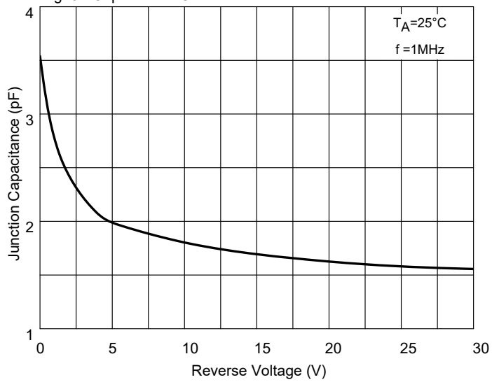
Fig. 3 - Capacitance Characteristics
