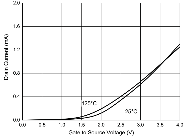
Fig. 2 - Transfer Characteristics
