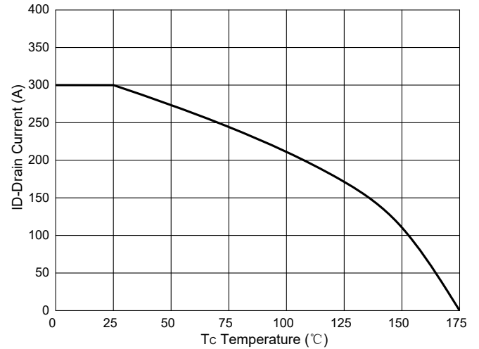
Fig. 10 - Drain Current
